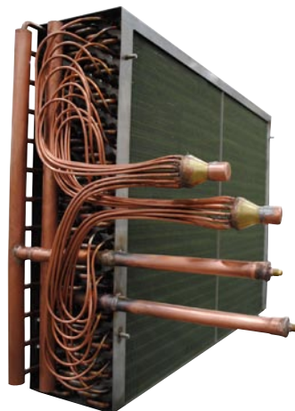
Evaporator with Pre-Coated Fins
